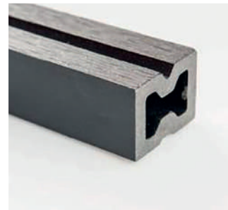
Rastrel de PVC 2200x40x30mm
